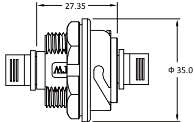
Connector Dimension
