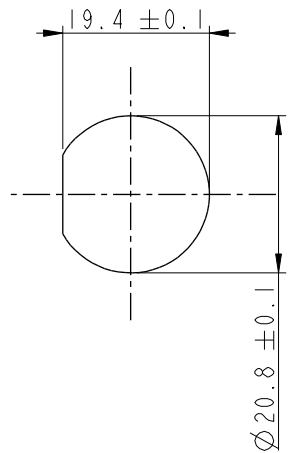
Recommended Panel Cut-out
