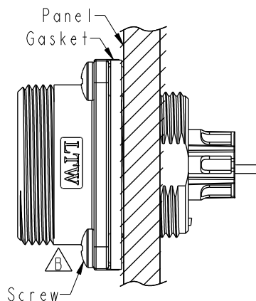
Assembly Instruction
