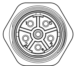
Conn. Pin Assignments Front View
