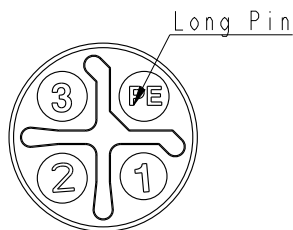
Pin Assignment Front View
