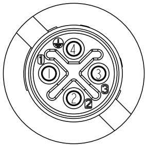
4P Pin Assignment Front View
