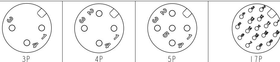
Pin Assignments Front View
