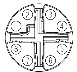
8P Pin Assignments Front View
