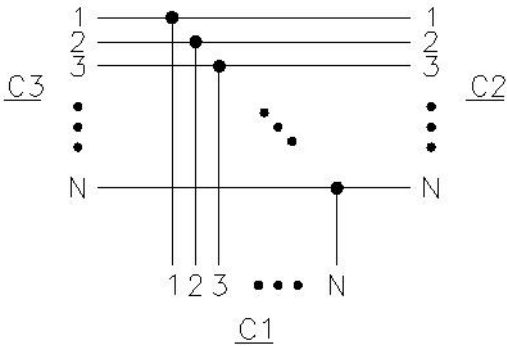
Connection Diagram
