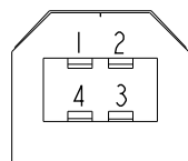
C1,C2 Pin Assignments Front View
