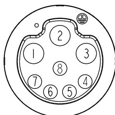
CI Pin Assignments Front View
