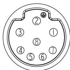
C2 Pin Assignments Front View
